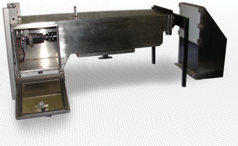
Washdown camera tube with backlight, enclosed CPU, and touchscreen
