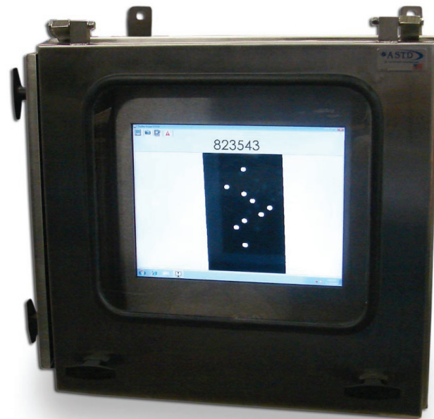
Washdown camera tube with backlight, enclosed CPU, and touchscreen
