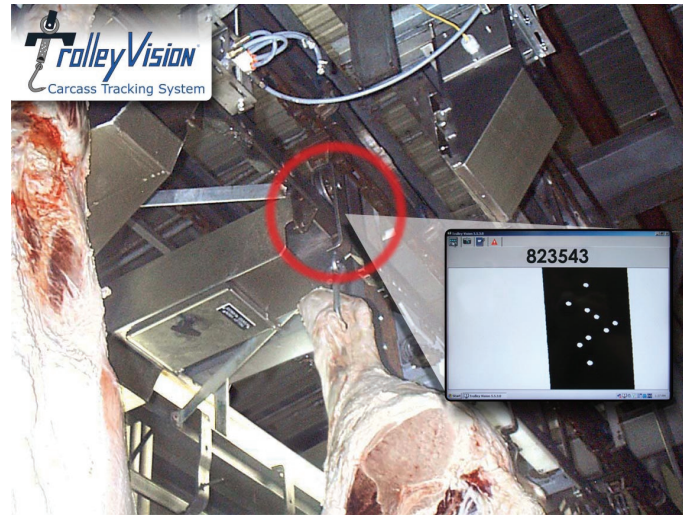
Carcasses tracked by Trolley Vision® for use in beef or pork applications
