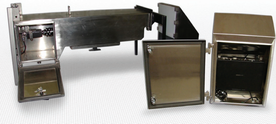
Washdown camera tube with backlight and enclosed CPU
